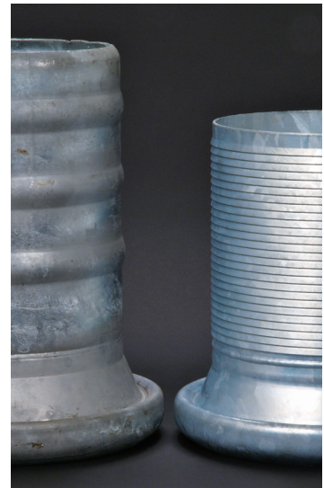
Bauer-style vs. Campbell Ball & Socket
