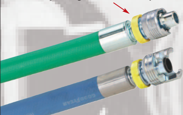
Use Campbell fittings with Nitrogen-Only Warning Rings on the hose and manifold to avoid deadly cross connections
